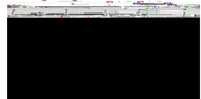
A G-quadruplex structure. Left (an intramolecular G 4 quadruplex) and right (a tetrad structure).
